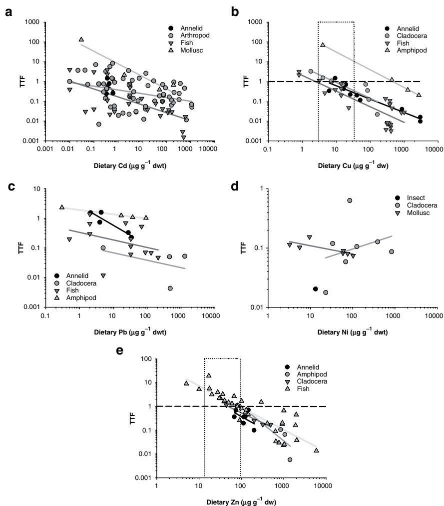
Fig. 1 Relationship between trophic transfer factors for different taxonomic groups and dietary exposure concentration from laboratory studies: (a) cadmium, (b) copper, (c) lead, (d) nickel, and (e) zinc. The horizontal dashed line indicates a TTF of 1. Solid lines represent regressions of TTF vs. dietary metal for individual taxa. The dotted boxes in (b) and (e) identify the range nutritional requirements for fish and some invertebrates (from Brown 2005)
