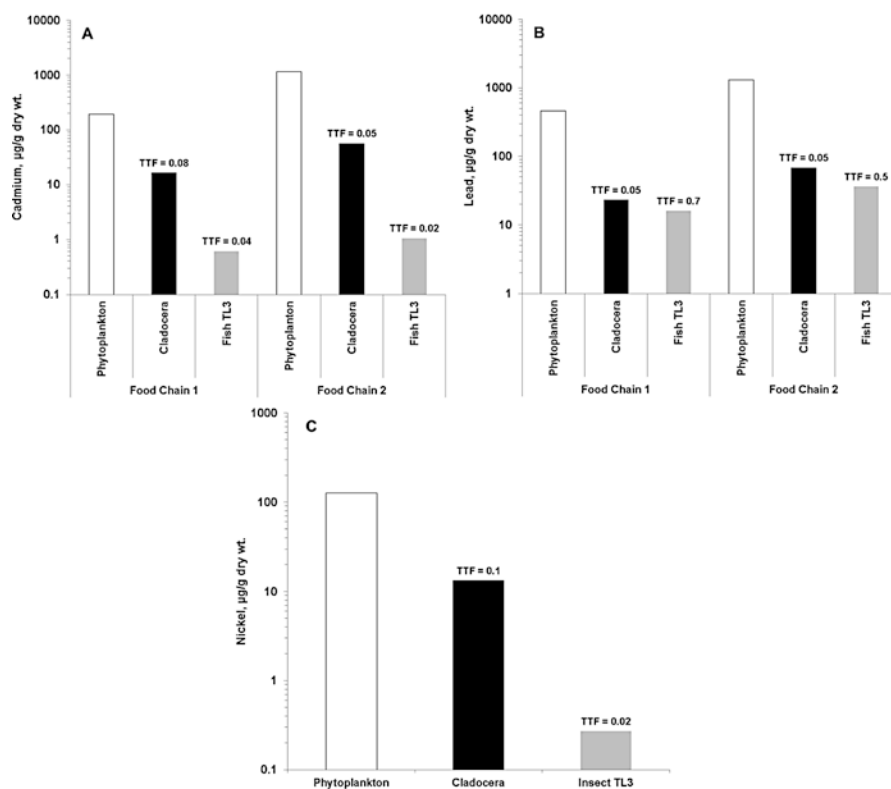
Fig. 3 Trophic transfer data from laboratory-simulated food chain studies for freshwater systems. (a) Cadmium, (b) lead, and (c) nickel. Geomean value for each taxonomic group. White bars =metal conc. in phytoplankton, Black bars =metal conc. in TL2, Light gray bars =metal conc. in TL3. Cadmium data from Ruangsomboon and Wongrat (2006); lead data from Vighi (1981); and nickel data from Ponton and Hare (2010)
